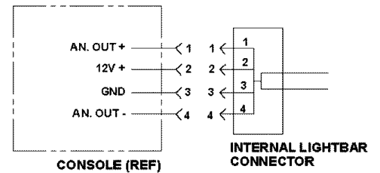
WIRING DETAIL
