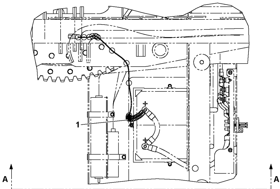
TOP VIEW OF BATTERY COMPARTMENT CAB REMOVED FOR CLARITY
