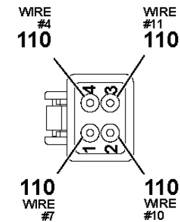
VIEW S - S SLEW POT INTERFACE CONN
