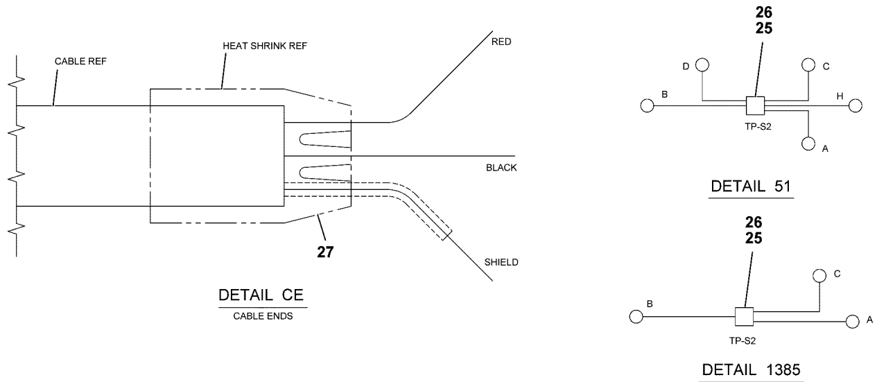
WIRE NUMBER LABELS FOR USE ON CABLE ASSYS
