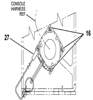
DETAIL-H DIAGNOSTIC CONNECTOR
