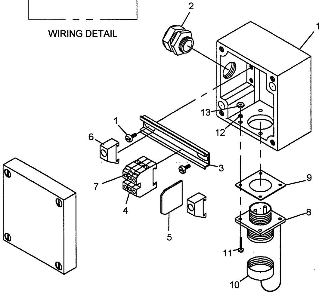
EXPLODED VIEW
