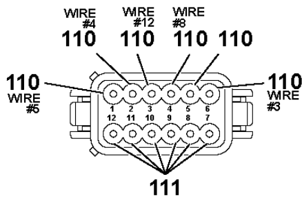
VIEW R - R CRANE INTERFACE CONN
