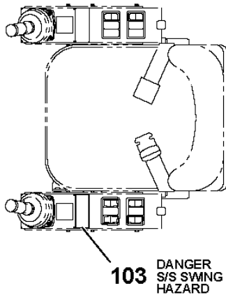
OPERATOR'S SEAT TOP VIEW
