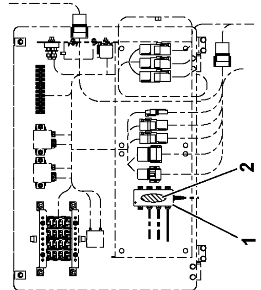
DETAIL B FUSE AND RELAY PANEL VIEW
