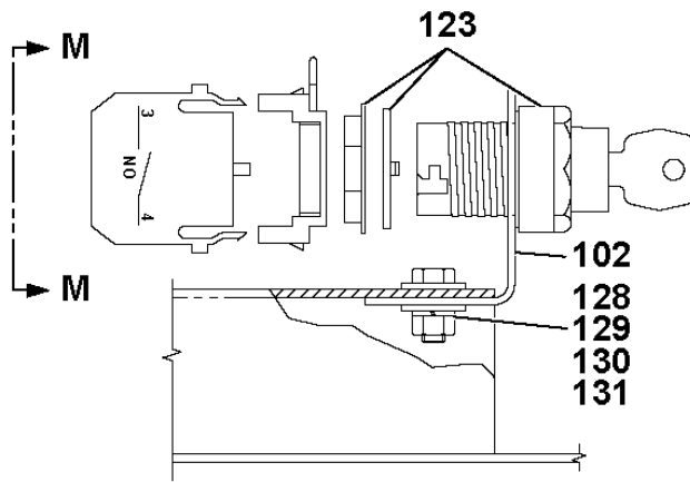
DETAIL K REAR BYPASS KEYSWITCH WIRES NOT SHOWN FOR CLARITY
