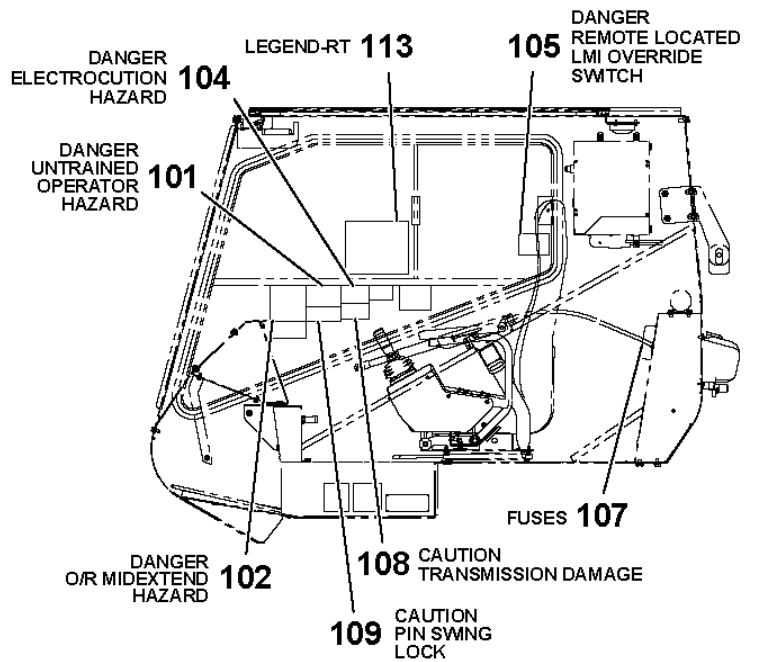
CAB LEFT INSIDE VIEW
