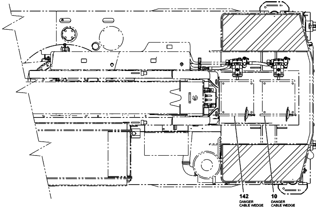
SUPERSTRUCTURE TOP VIEW
