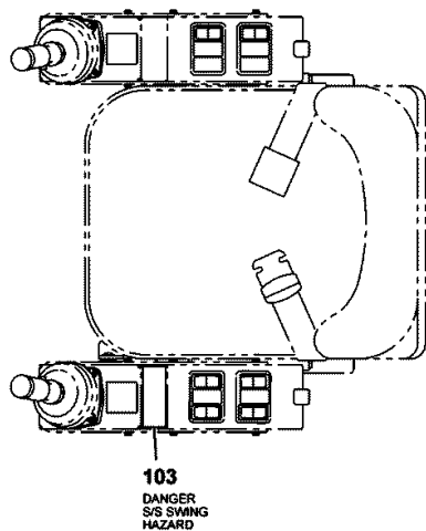
OPERATOR'S SEAT TOP VIEW
